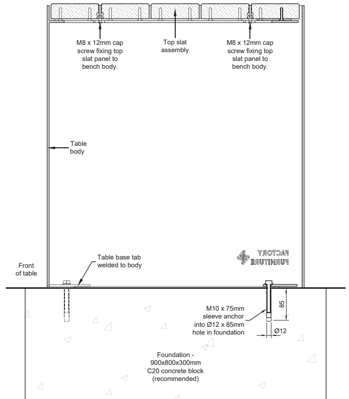
X-Section Thro' Table
